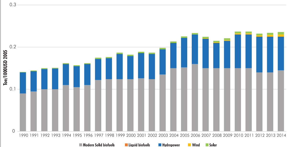
FIGURE 8 CONSUMPTION OF MODERN RE SECTORS IN THE ARAB REGION DOMINATED BY BIOMASS AND HYDROPOWER
